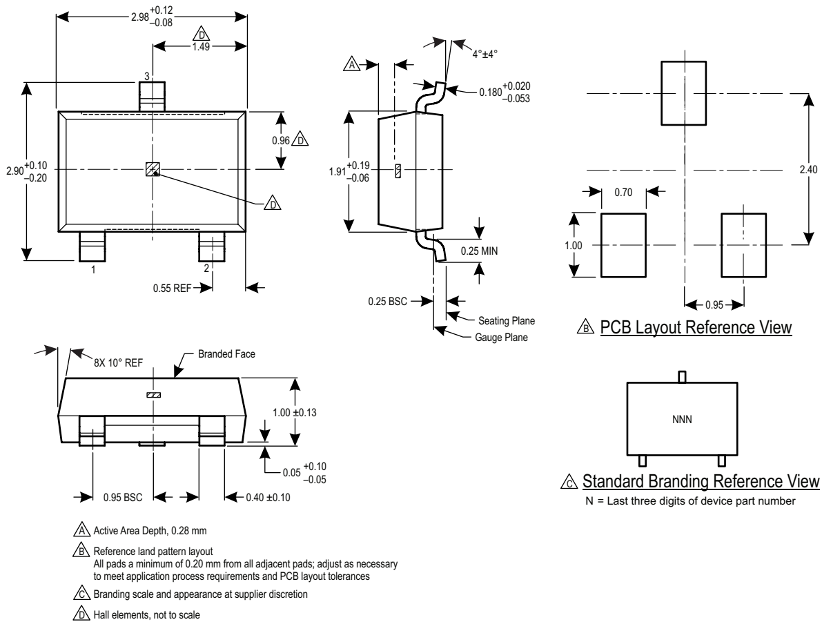
Figure 3: Package LH, 3-Pin SOT-23W
