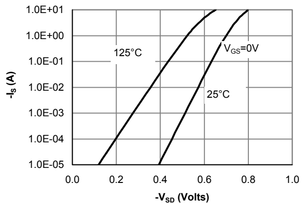
Figure 6: Body-Diode Characteristics
